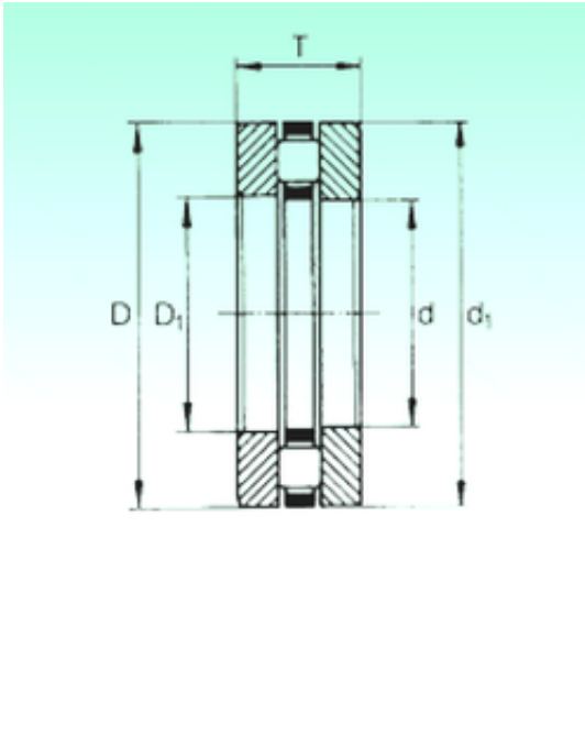
81134TN Bearing 2D drawings and 3D CAD models
