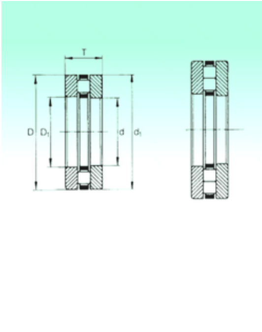
89413TN Bearing 2D drawings and 3D CAD models
